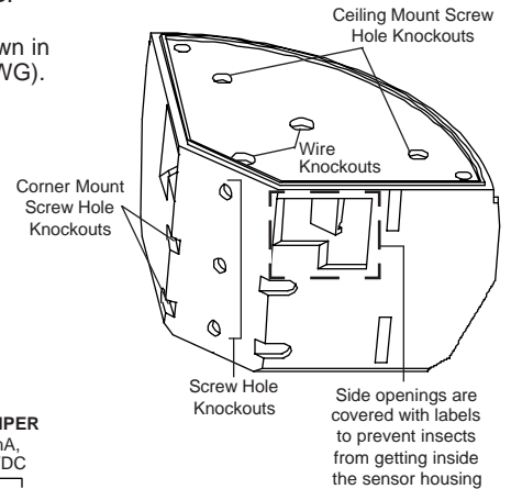
Figure 2 Rear Housing
