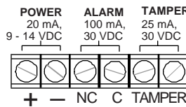
Figure 3 Wiring
